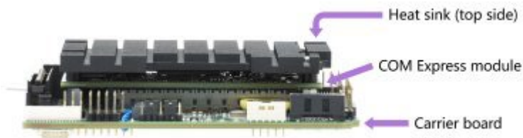
A COM-based SBC consists of 3 elements: carrier board, COM, and thermal solution
