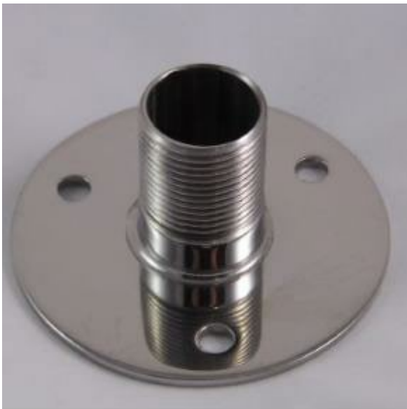
6538S Universal mount stainless steel. Standard thread 1" x 14, weight 150 grams. Height 41.275 mm. (1.625")
