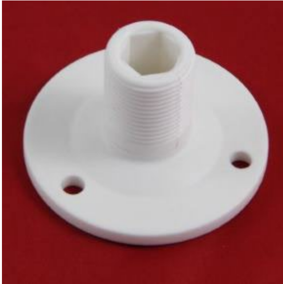
6538N Universal mount reinforced nylon. Standard thread 1" x 14, weight 50 grams. Height 41.275 mm. (1.625")
